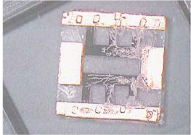
Figure 5. Peak power exceeds power limit
