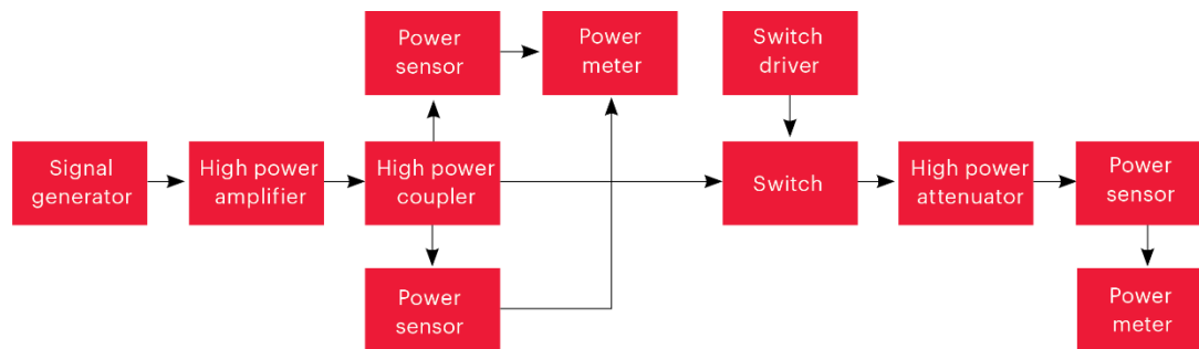
Figure 6. Power handling test setup
