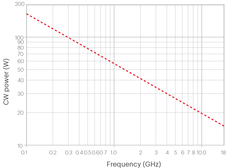
Figure 2. Power rating for cold switching
